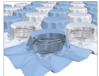
Alternating coil design
